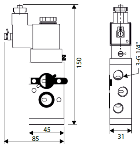
5/2 Configuration
